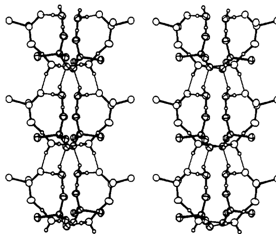
Fig. 2. Stereoview of (\text{C}_6\text{F}_5)_2\text{PO}_2^- \text{H}_3\text{O}^+ showing the H-bonding network. The perfluorophenyl groups are omitted for clarity.
