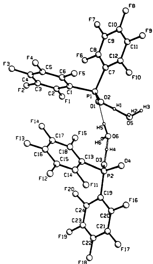
Fig. 1. Structure of (\text{C}_6\text{F}_5)_2\text{PO}_2^- \text{H}_3\text{O}^+ showing the atom numbering scheme.
